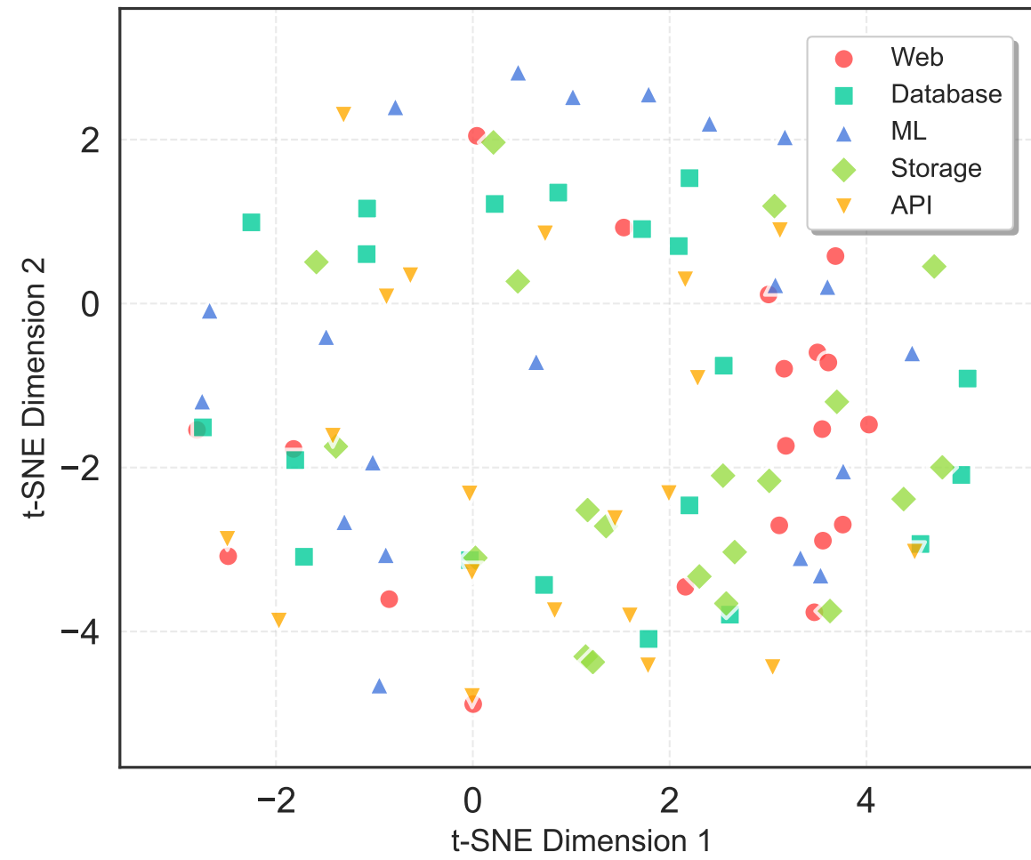
RandomPlacement Semantic Embedding Clusters
